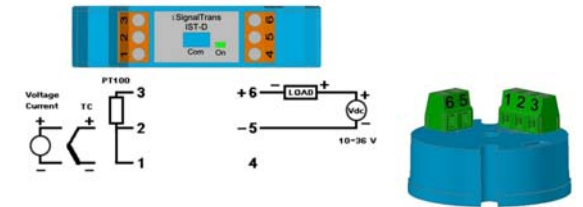
Figure 2. Terminal connections
